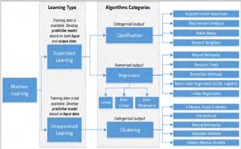
Figure 3.4: Machine Learning Types: Source: [Batinca and Treleven, 2014]
